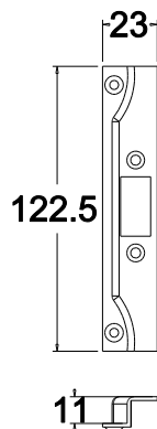
Rebated Forend
