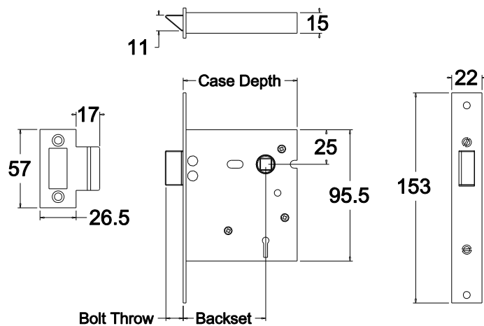
Bolt Throw
