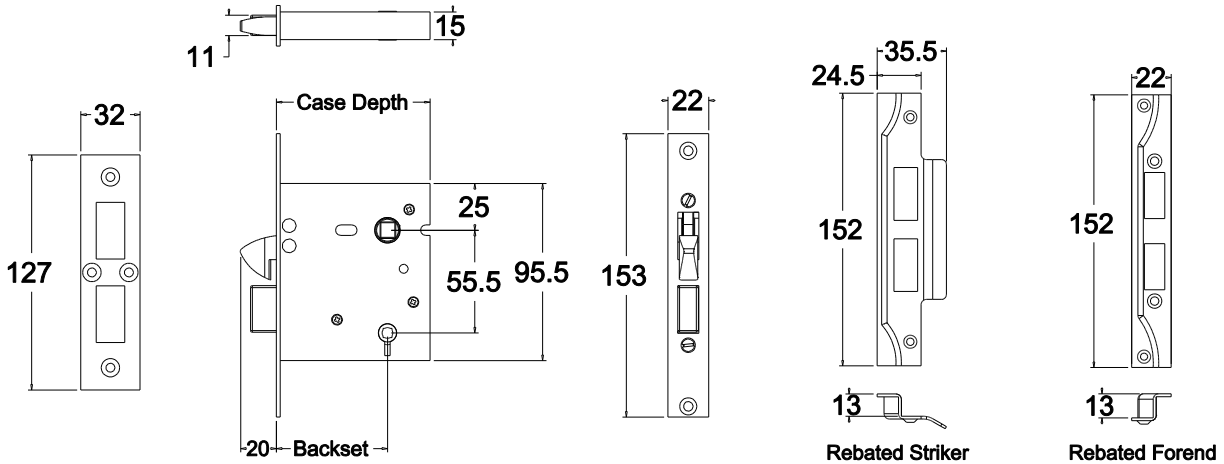
JM160SL Sliding
