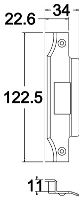
Rebated Striker
