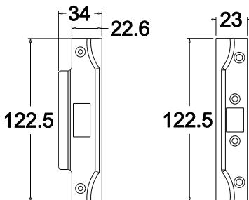
Rebated Forend
