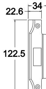
Rebated Striker
