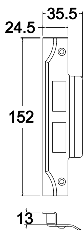
Rebated Striker
