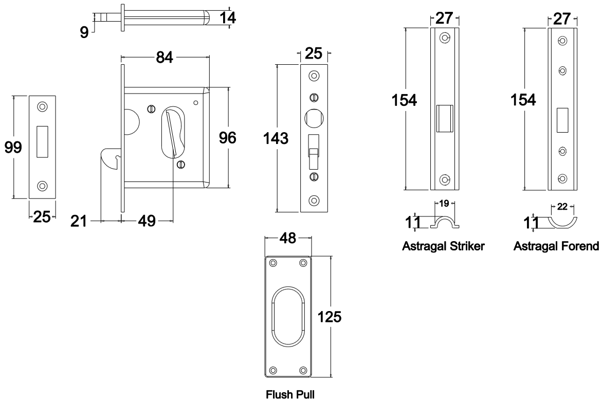
FLUSH PULLS 125mmx 48mm (4 supplied with JM32A)
