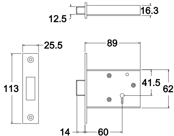
Rebated Forend
