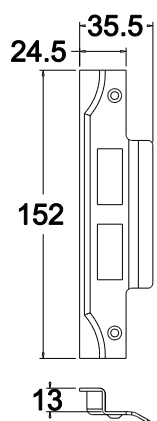
Rebated Striker
