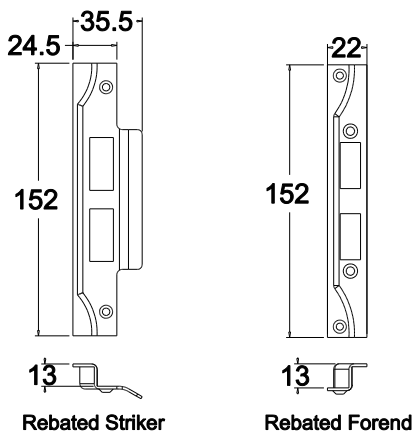
JM560R Rebated
