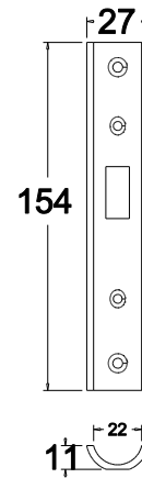
Astragal Forend
