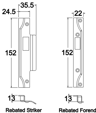
Rebated Striker
