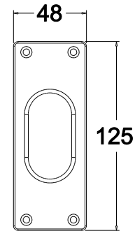
Flush Pull
