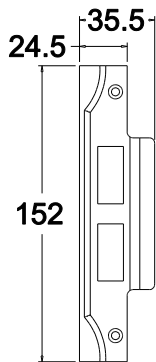
Rebated Striker
